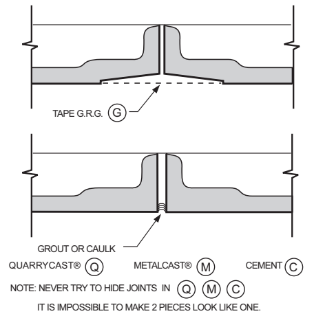
④ JOINT DETAIL
