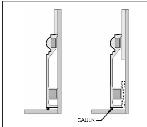
CONDITIONS WITH QUARRYCAST® VENEER
