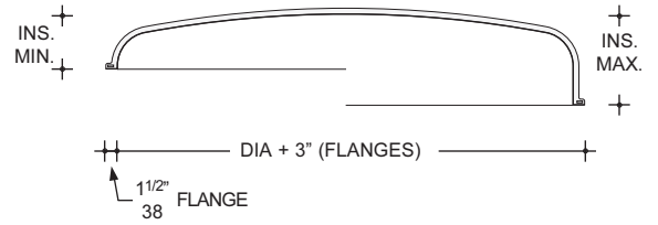
DOMES [SERIES #70100]
