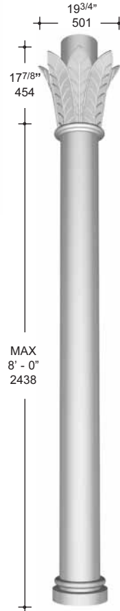
SHAFT 8" 203 #18908
