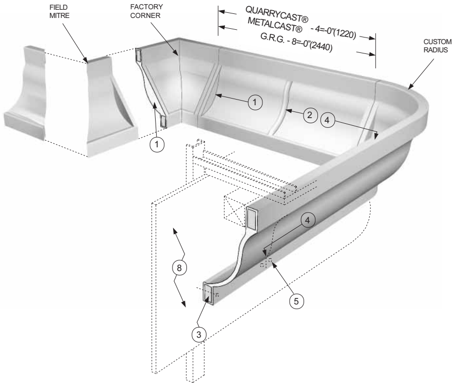
④ JOINT DETAIL
