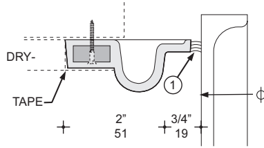
DRYWALL BULLNOSE
