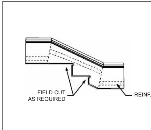
CONDITIONS AT STAIRS - FIELD CUT
