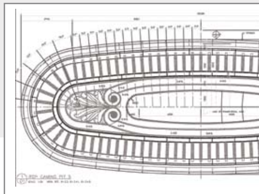
Formglas Drawing
